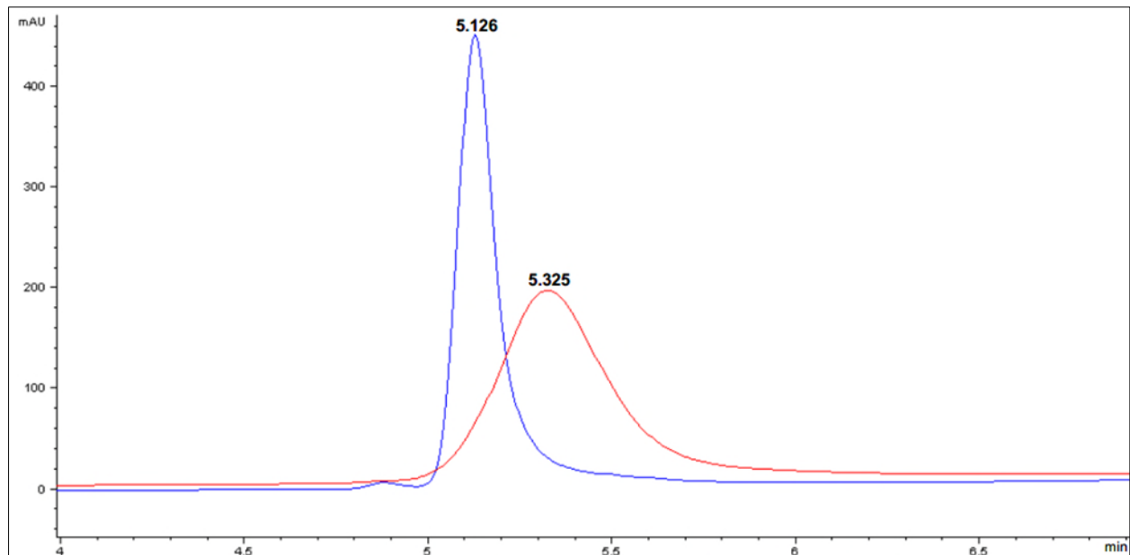
Figure 2. Overlay of C4 Reversed phase analysis of BSA (before labeling, blue trace) and Maleimide Activated BSA LL (after labeling, red trace showing absorbance at 220 nm).
