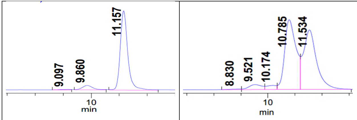
Figure 1. Size exclusion HPLC profile of BSA(beforelabelling, left) and purified conjugate Maleimide Activated BSA LL (right)
