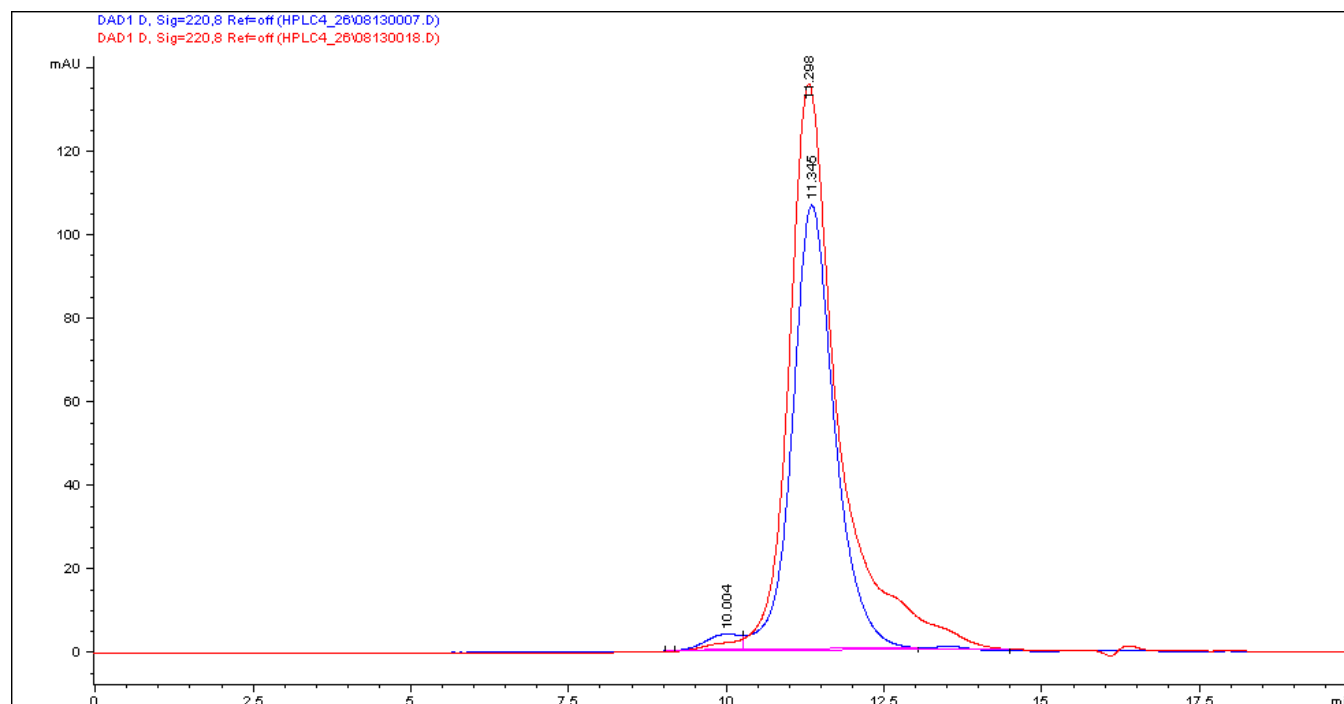
Figure 1. Representative size-exclusion HPLC profiles of Biotin Goat Anti-Human IgG (H+L) before labeling (blue trace; ~3% aggregation, indicated by the peak at 10.004 minutes) and after AqT® biotin labeling (red trace). The biotinylated antibody (Lot No. S715.S9.0814F; DOL: 2.8) demonstrated ≥99% monomeric purity in PBS, with no detectable aggregate peak.
